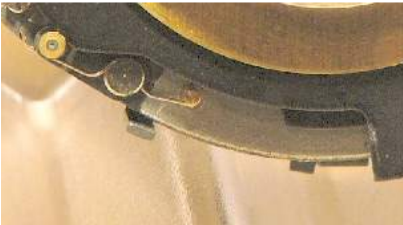
PIC 7: Diaphragm roller (lens cocked)
