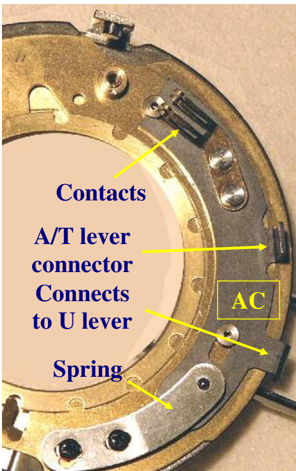
PIC 42: A/T slide AC
