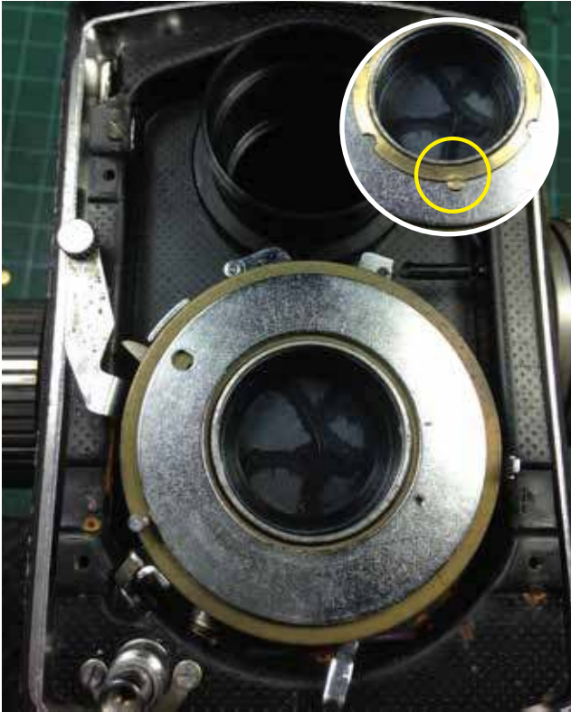
01: Unscrew the small screw (Highlighted HL in yellow) in inset photo. Do note when putting it back DO NOT over-tighten. And remove the cover plate retaining ring using only your fingers. If its too tight use the lens spanner. Be gentle as the materials are thin metal.
