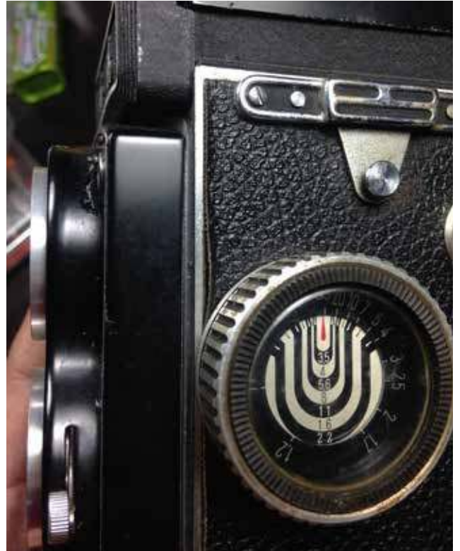
08: Before removing the front plate, make sure you make notes of the distance, speed and aperture setting. Ideally put the speed to B, aperture to the widest opening (3.5) and distance scale to infinity.
