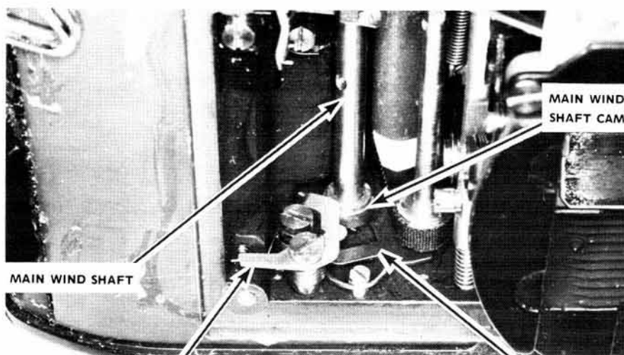
OPENING CURTAIN BRAKE LEVER
