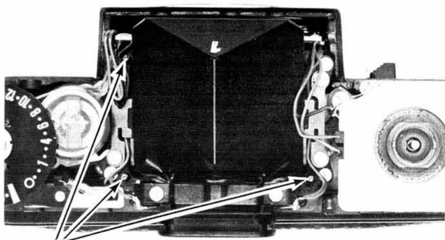
FOCUSING SCREEN ADJUSTING SCREWS
