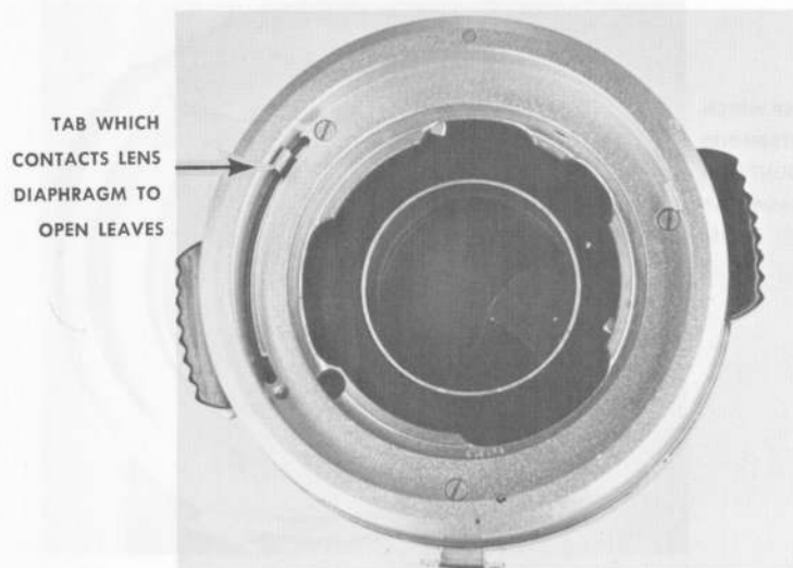
SHUTTER RELEASED
