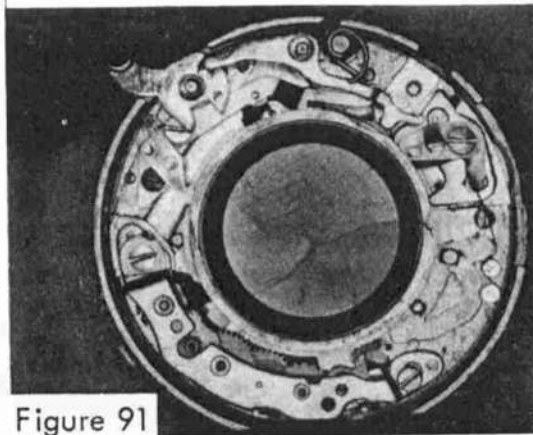
Removing the Cable Release Lever
