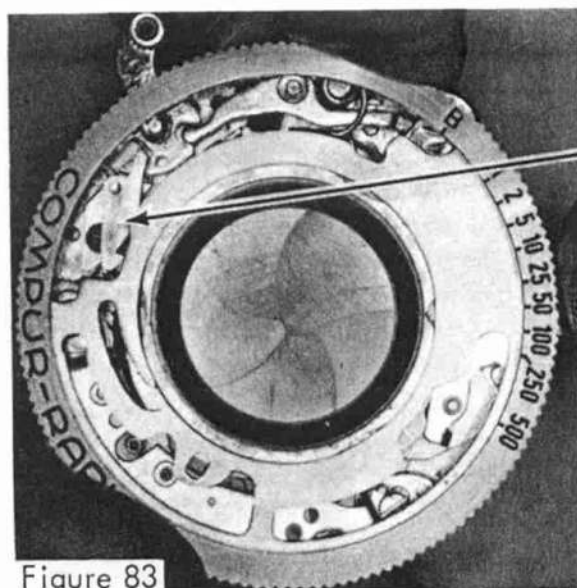
Inner Release Lever
