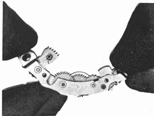
Unwinding the Hair Spring
