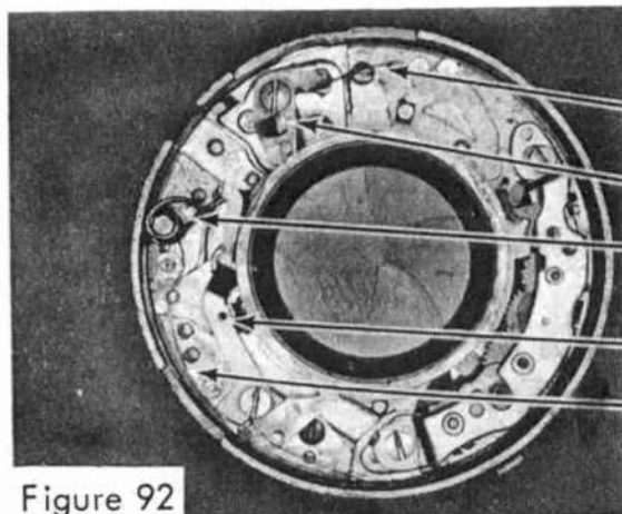
Leaf Lever Spring Leaf Lever High-Speed Spring Bulb Lever Bulb Lever Spring
