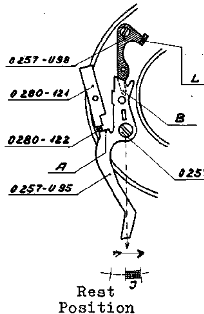
Fig. 2a (Size 0 Shutter)
