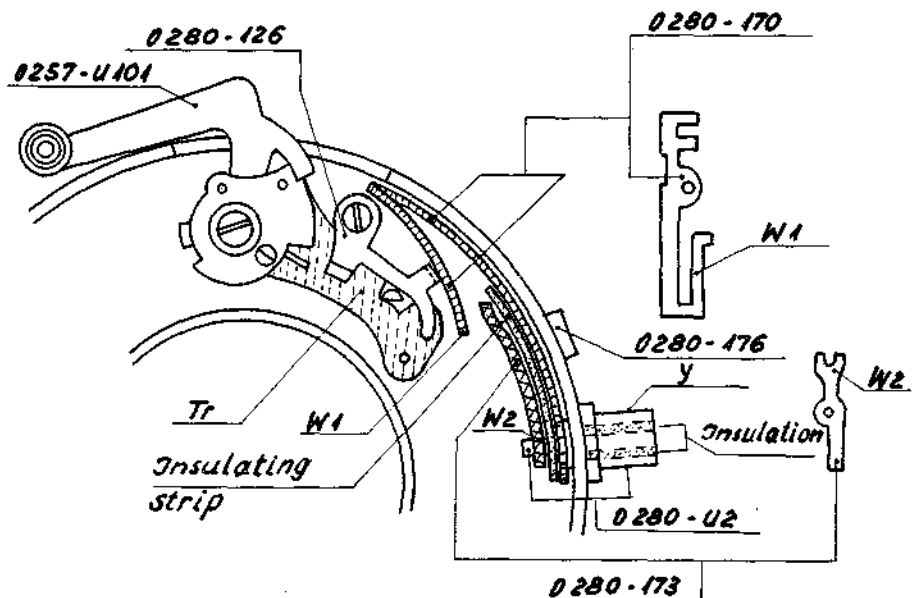
Fig. 7a (Size 0 Shutter)
