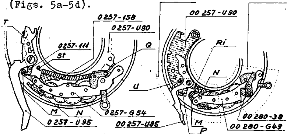
Fig. 5a (Size 0 Shutter)
