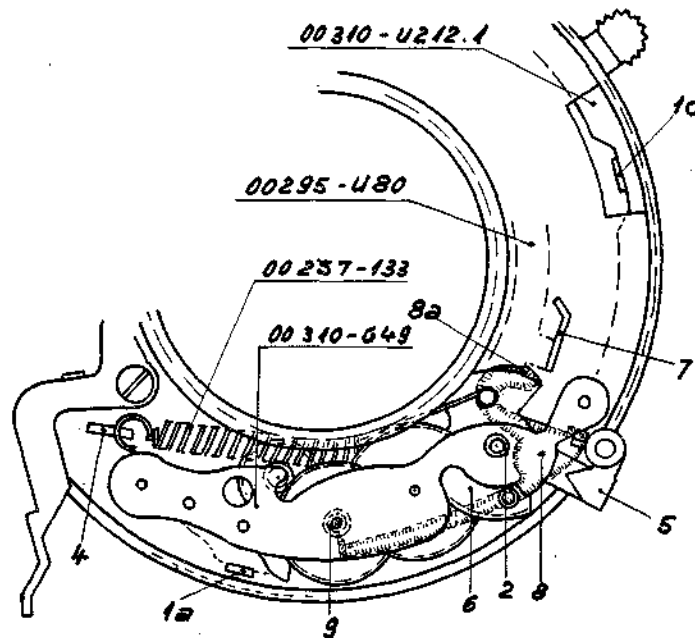
Fig. 10a (Size 00 Shutter) 00257-133 Spring of Delayed Action Device 00295-U80 Shutter Drive Ring 00310-G49 Delayed-Action Device 00310-U212.1 Synchro Switch Ring
