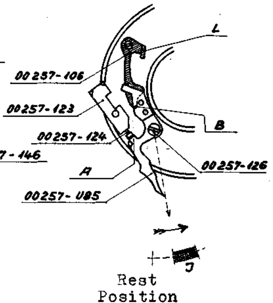
Fig. 2b (Size 00 Shutter)
