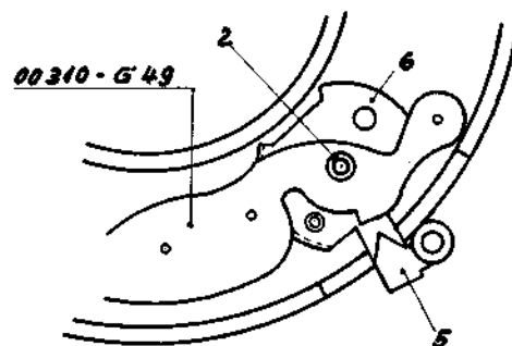
Fig. 9 (Size 00 Shutter)
