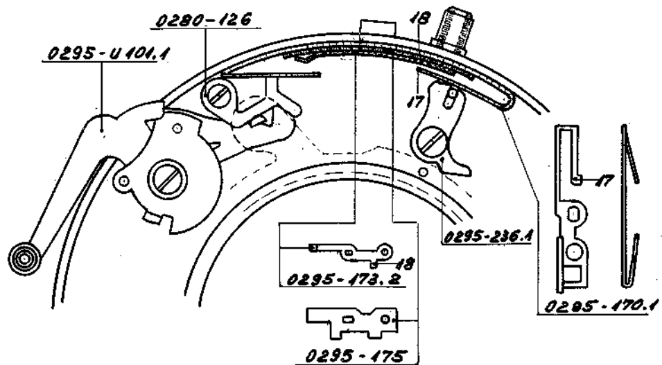
Fig. 11c (Size 0 Shutter)
