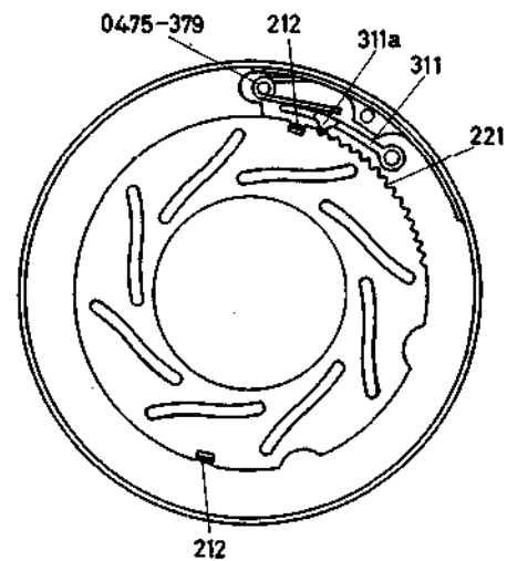
Fig. 34 - Diaphragm Cover Plate with Detent Lever
