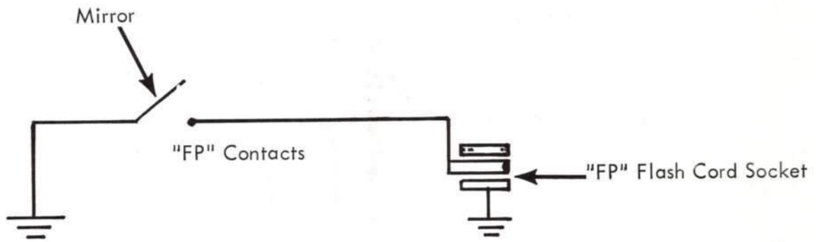
A. "FP" Flash Circuit
