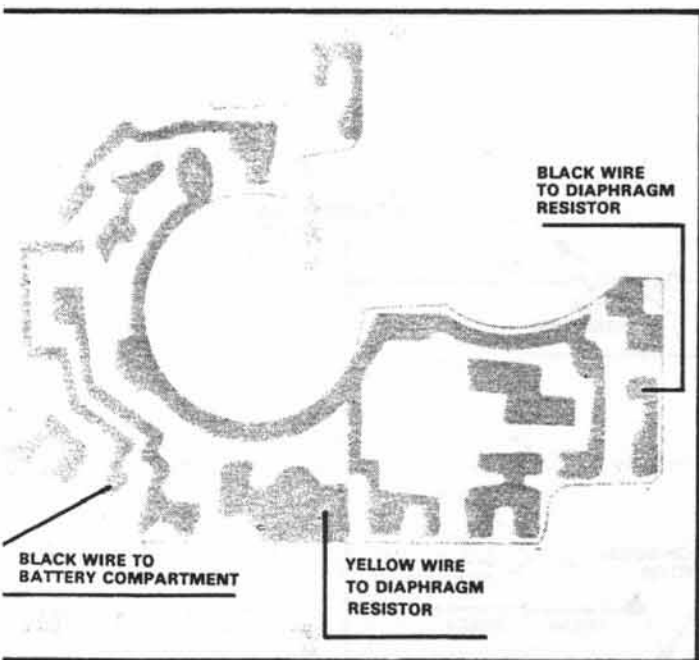
Figure 75 Exposure-meter circuit board
