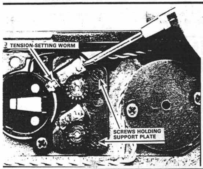
Figure 166 Removing the closing-curtain tension-setting worm
