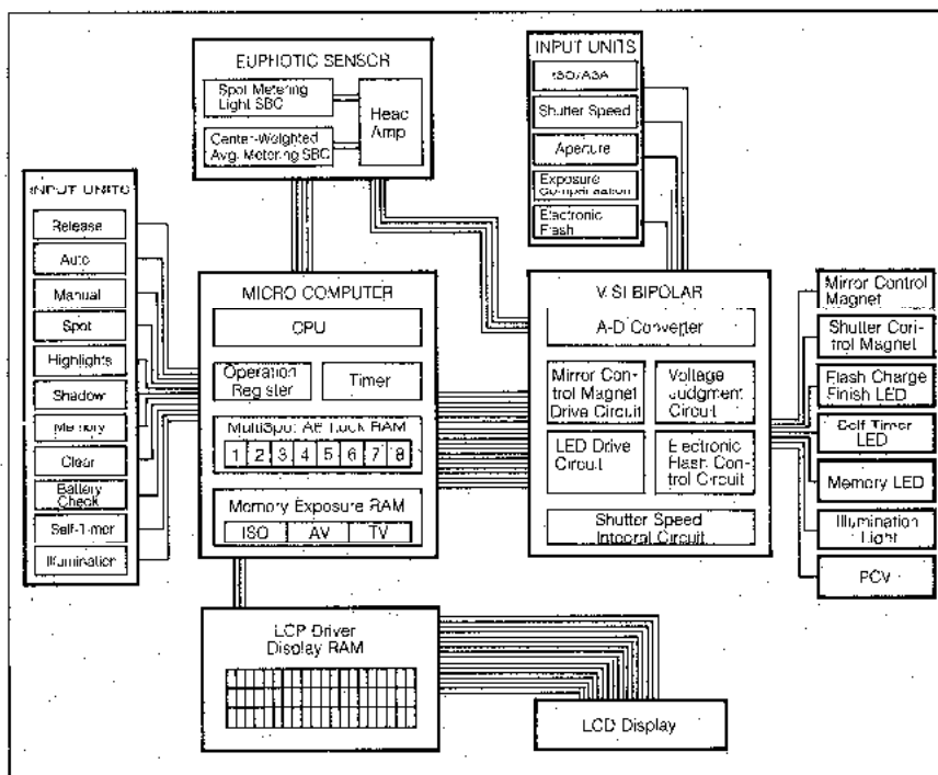
The OM-4's Electronic Heart: The camera's innovative IC system for exposure control, diagrammed for clarity.
