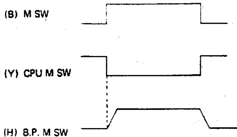
Time chart
