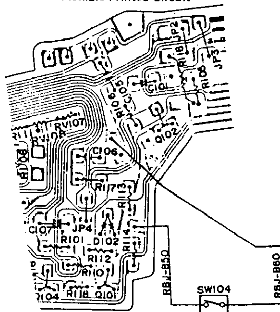
Flexible Printed Circuit
