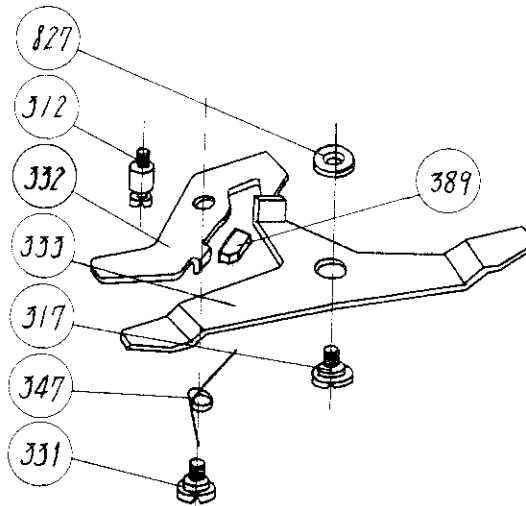
Mirror support
