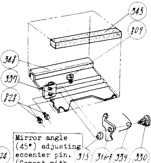
Mirror box, inside
