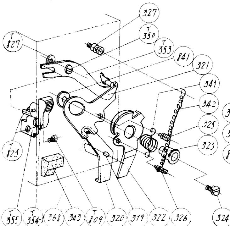
Mirror box, right
