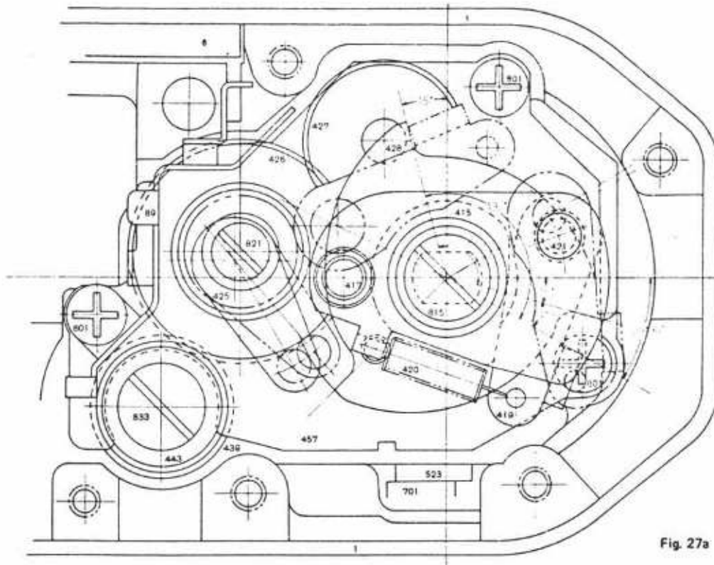
Charge cam and Advance gear
