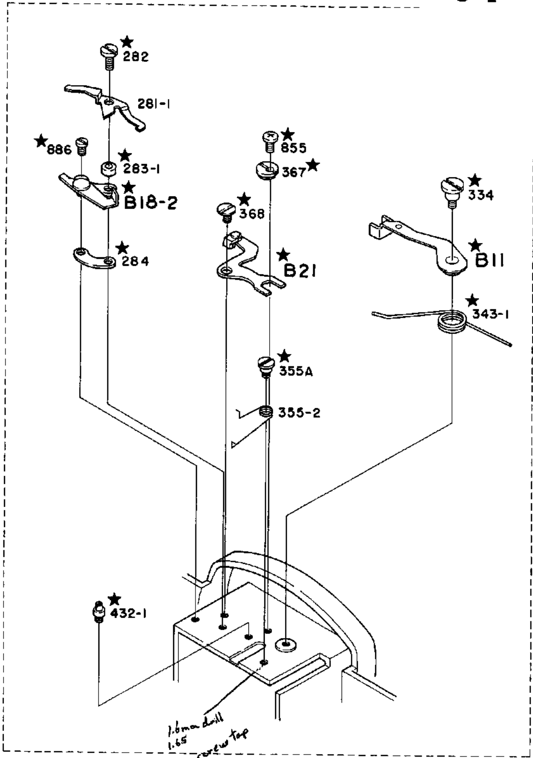
Jig 15 J15160
