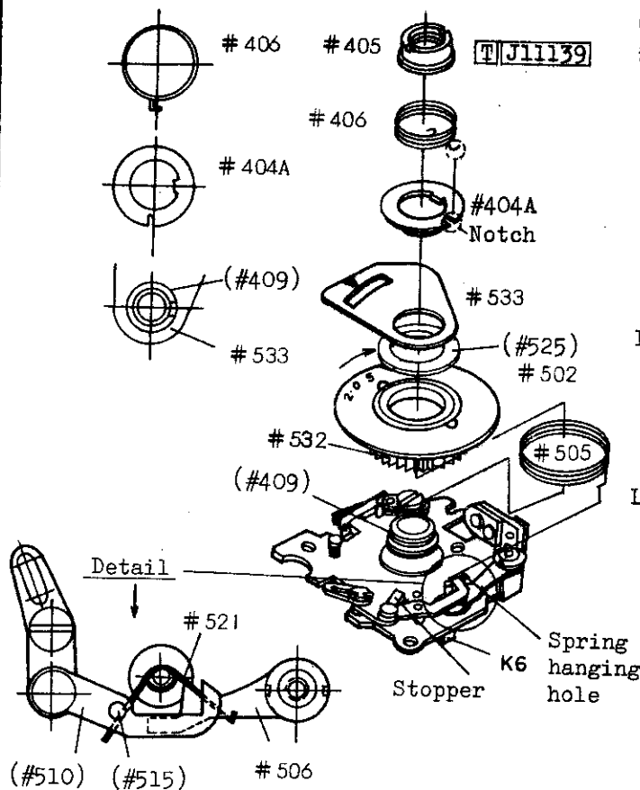
Hanging position of spring #521
