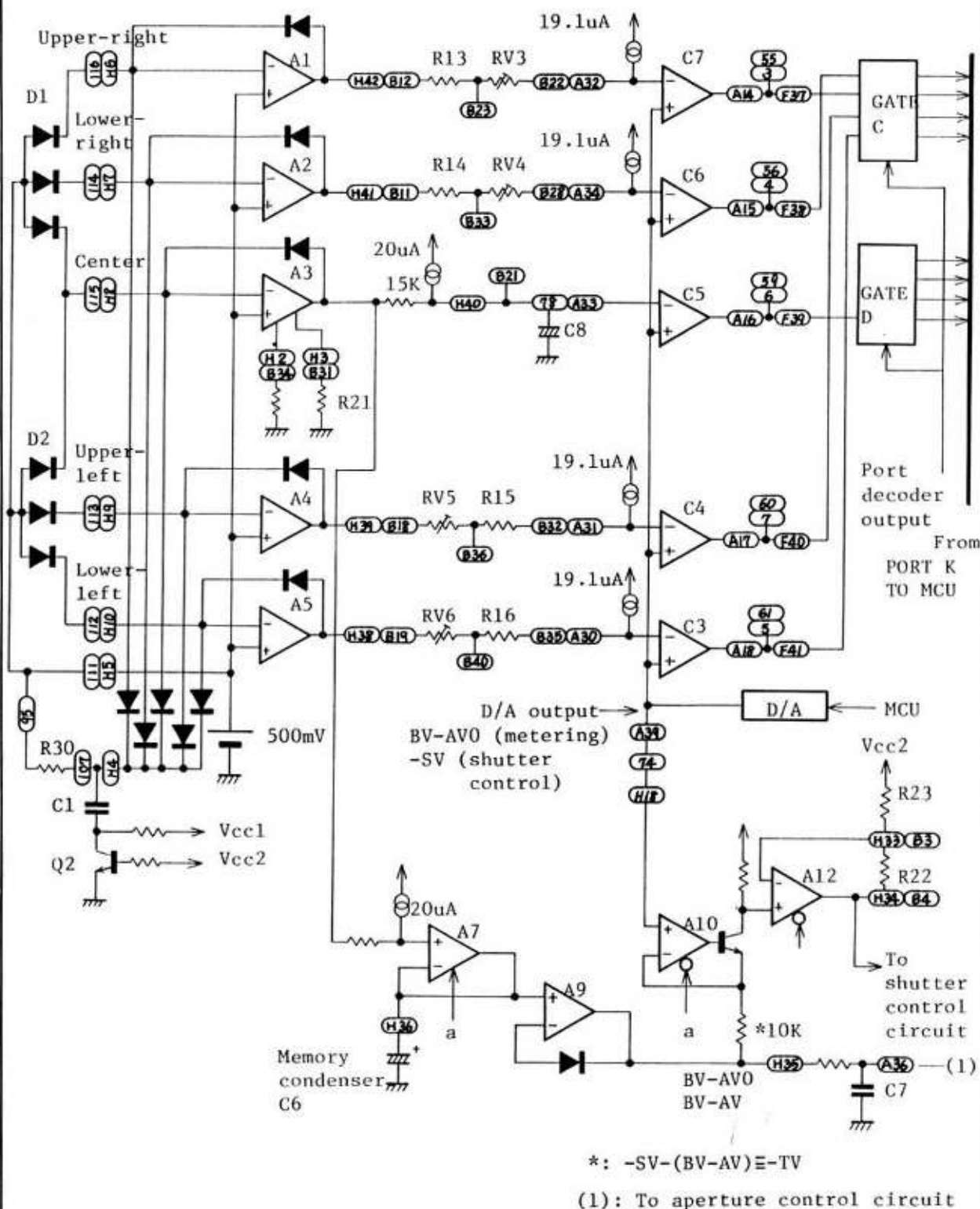
Figure 3 Metering circuit block diagram
