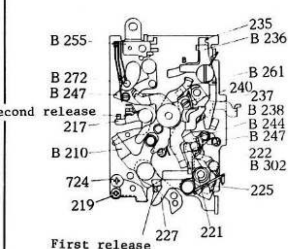
9-3 MIRROR SWITCH ADJUSTMENT
