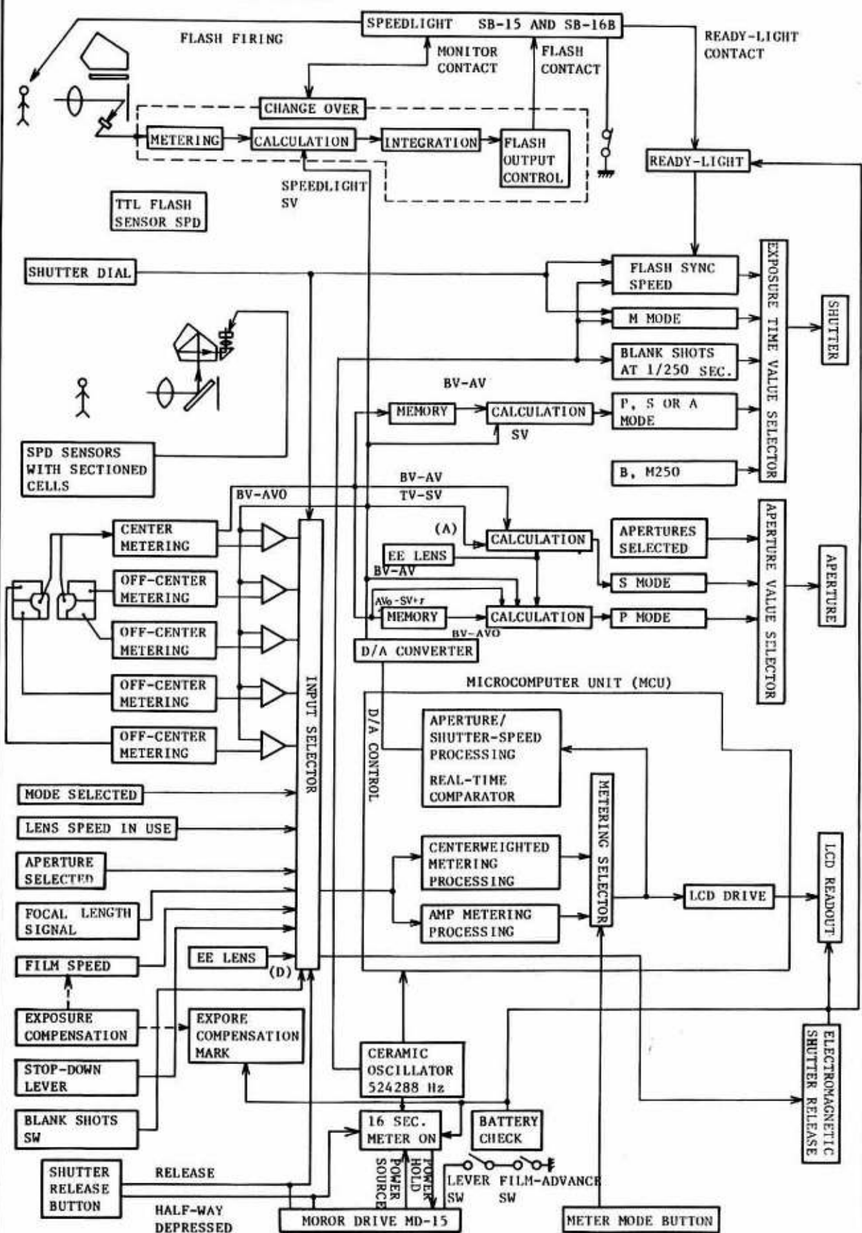
CAMERA OPERATION BLOCK DIAGRAM
