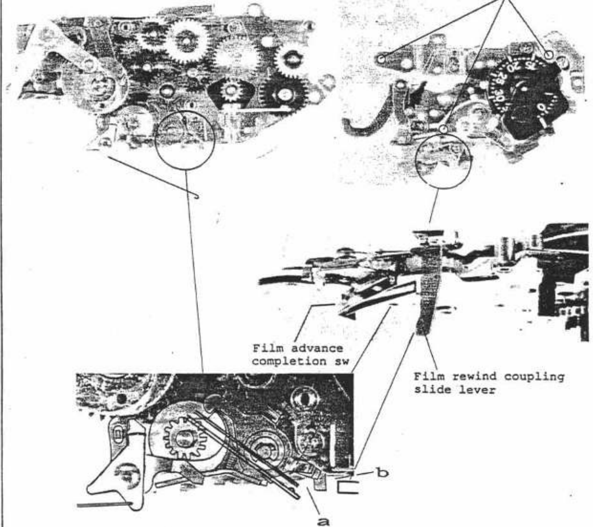
Upper film advance unit
