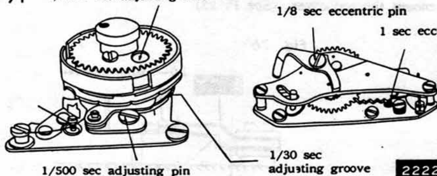
Fig. 71 1/1000 sec adjusting hole
