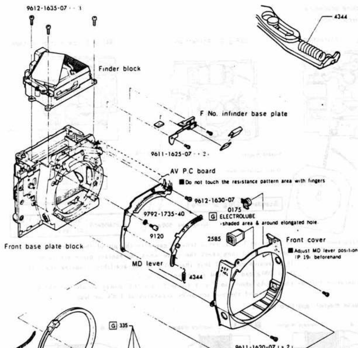
Fig. 1 4344 spring setting
