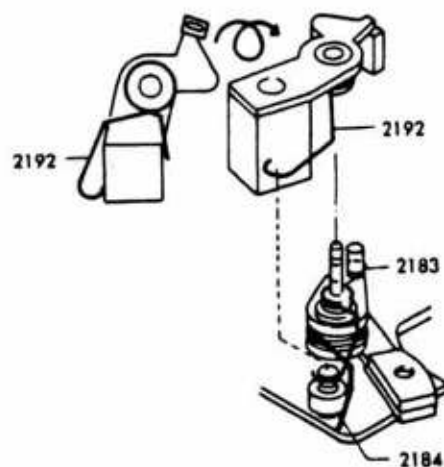
Fig. 3 2183, 2184, 2192 spring setting
