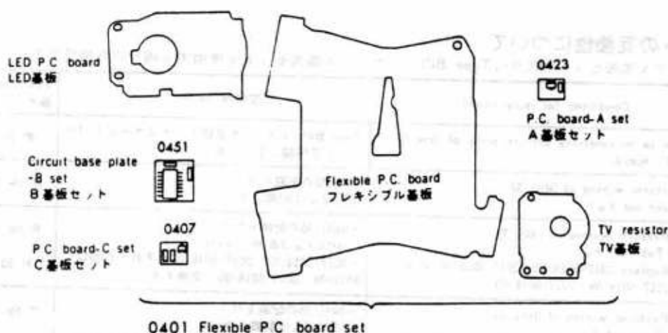
0401 Flexible P.C. board set
