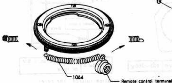
Fig. 2 1064 spring setting
