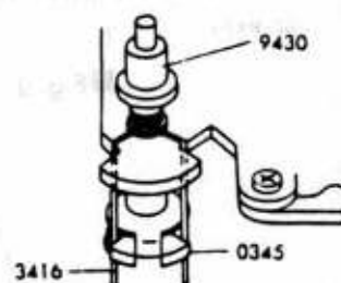
Fig. 2 3416 spring setting
