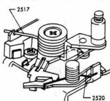
■ Fig. 2 2517, 2520 spring setting
