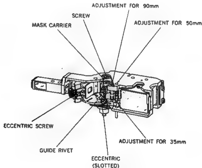
Figure 4-22. Range-Viewfinder Adjusting Points.
