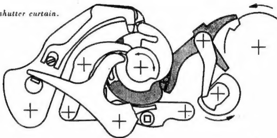
Figure 1-6. Controls in "B" Position, Shutter Released.
