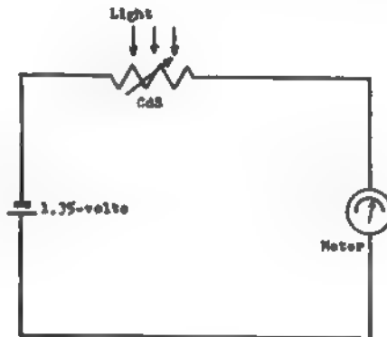
Figure a. Light Measuring Schematic.
