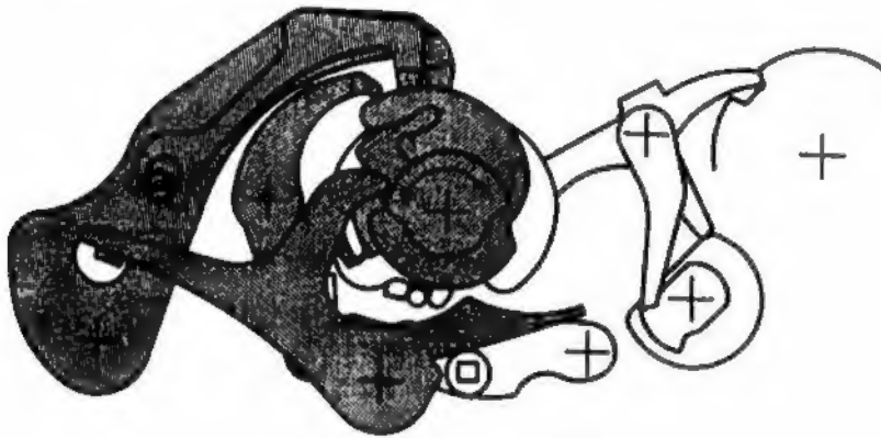
Figure 1-8. Controls in 1/1000-Second Position, Shutter Wound.
