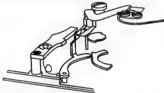
Figure 1-14. Flash Bulb Circuit, Contacts Closed.
