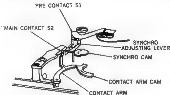
Figure 1-13. Flash Bulb Circuit, Contacts Open.
