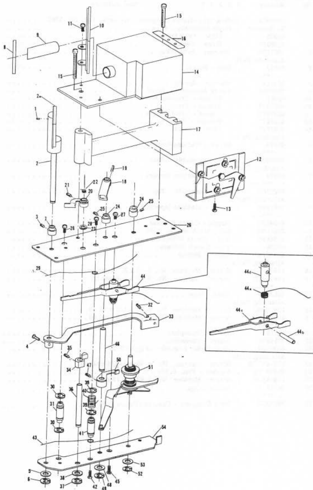
Figure 2-2. RANGEFINDER ASSEMBLY
