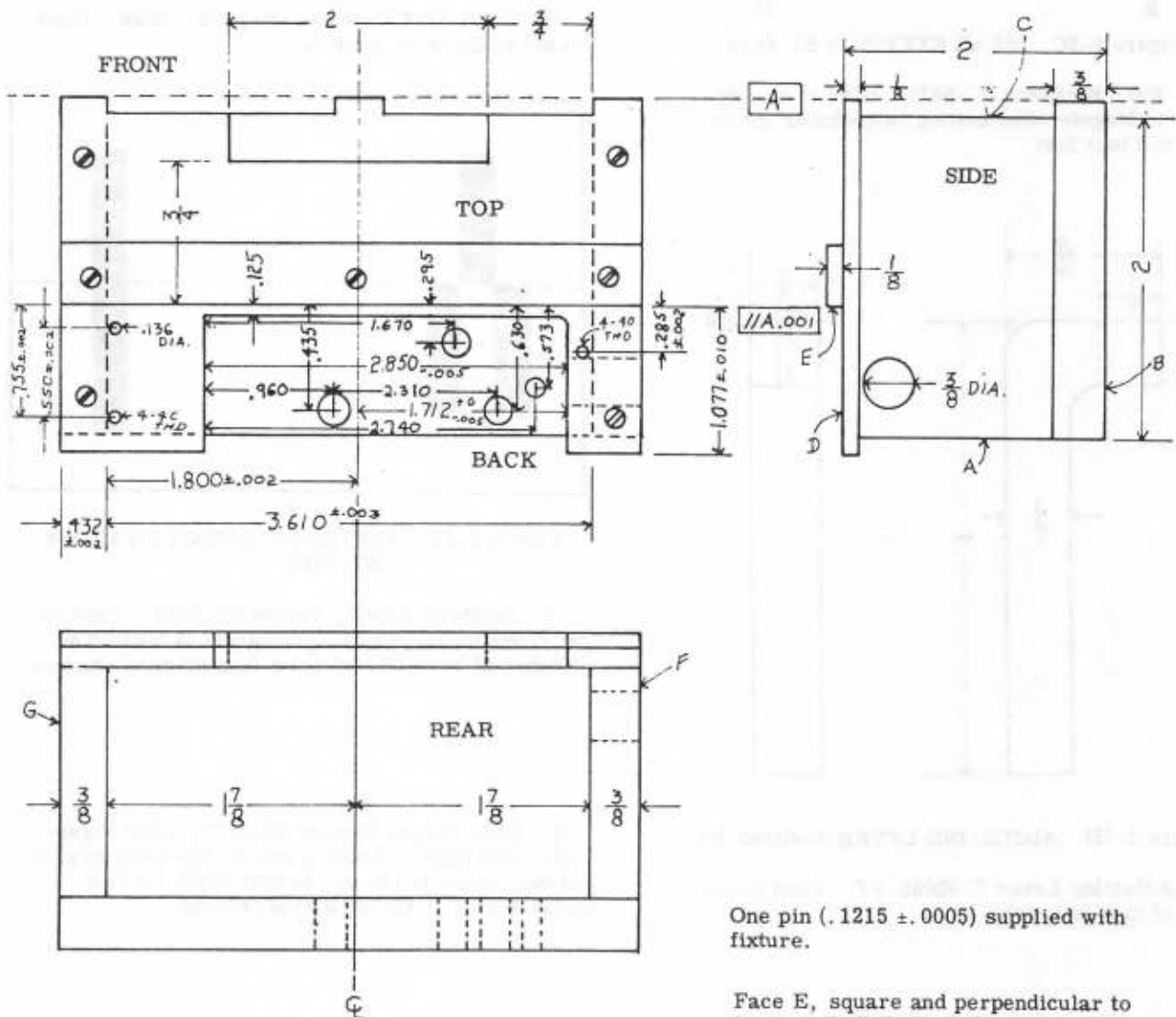
Figure 1-2B. RANGEFINDER ASSEMBLY ENGAGING FIXTURE ST-6636
