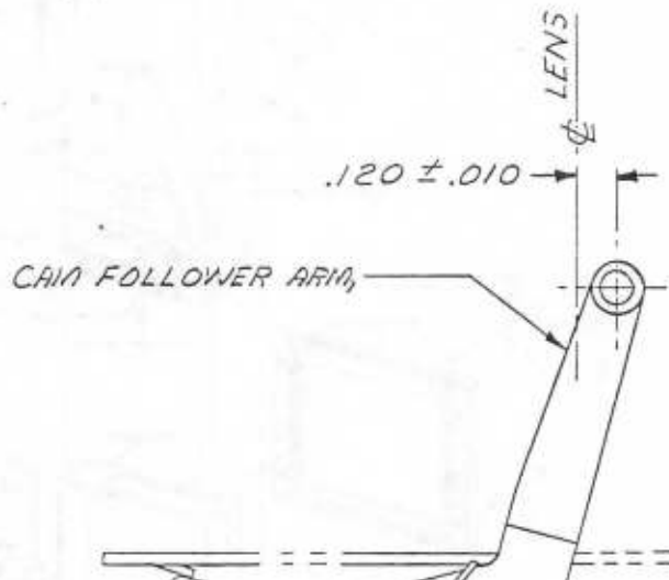
Figure 1-11A. FOLLOWER ARM SETTING
