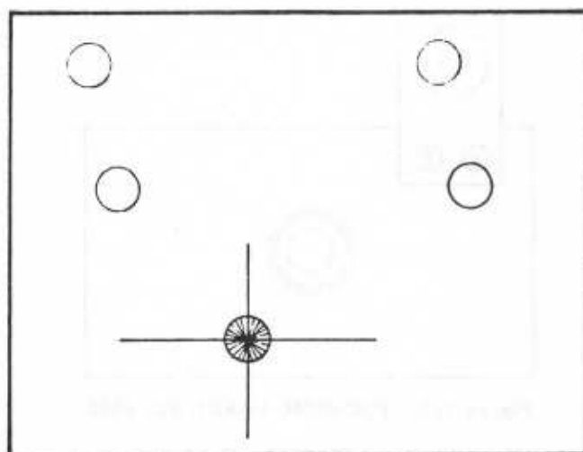
Figure 1-2E. FOUR FOOT PARALLAX TARGET ST-6638
