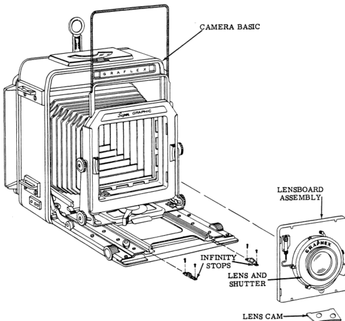
Figure 1. CAMERA COMPLETE
