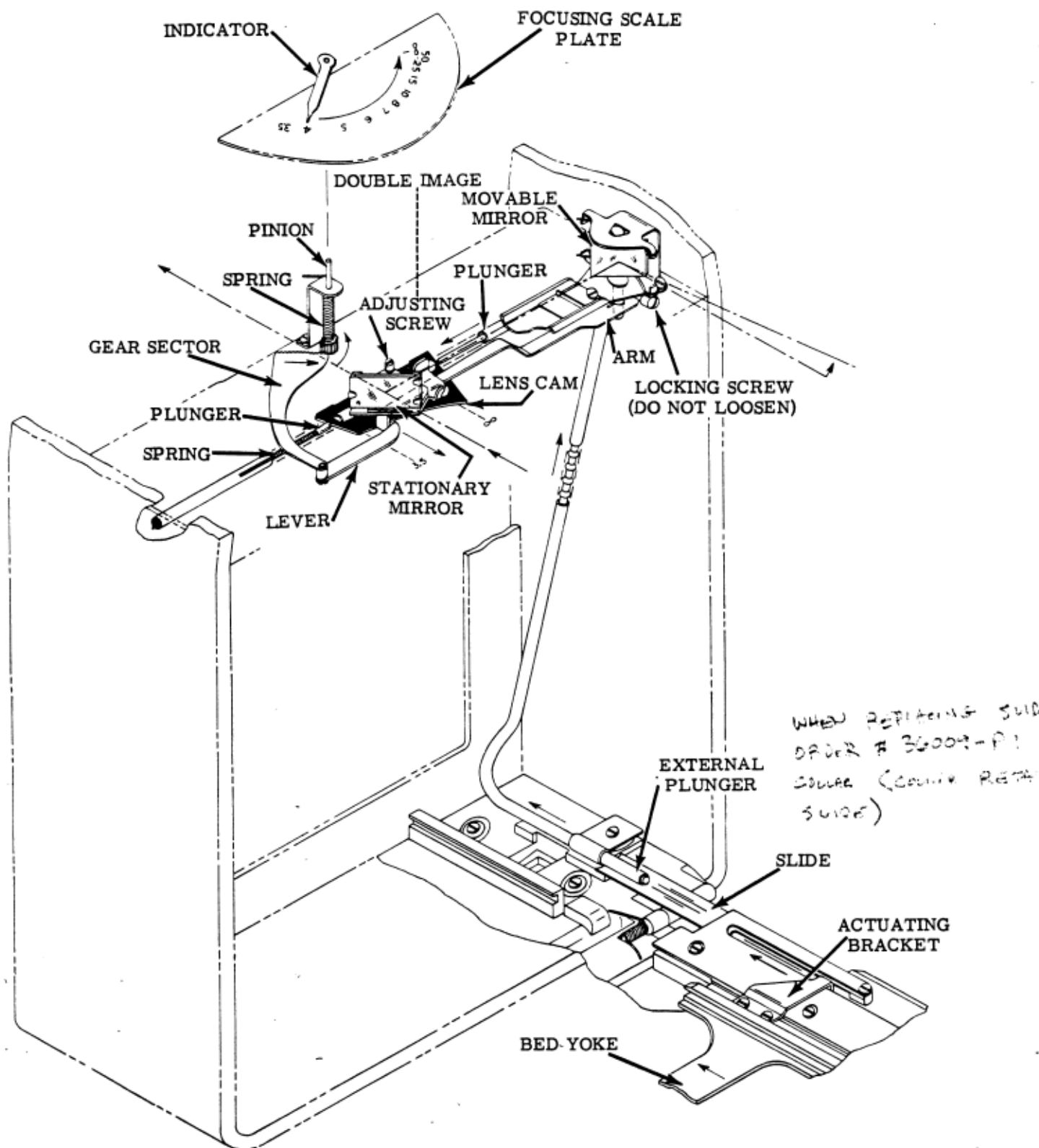
Figure 2. RANGEFINDER OPERATION
