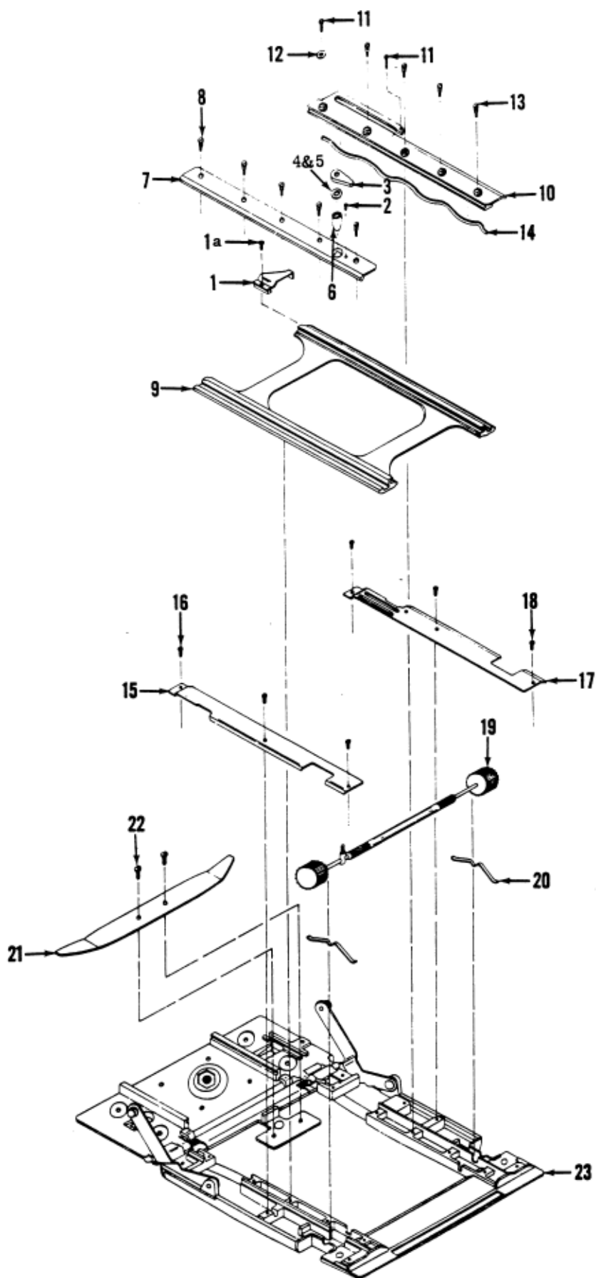
Figure 11. BED COMPLETE
