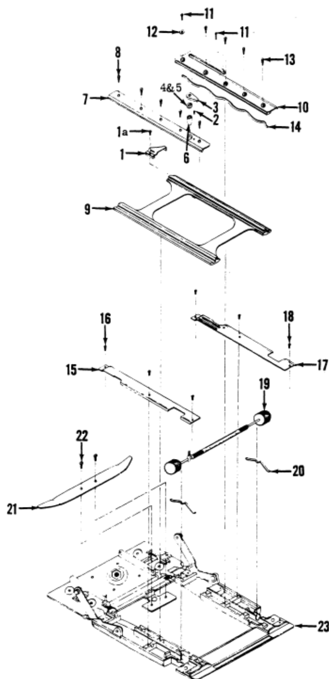
Figure 6. BED COMPLETE
