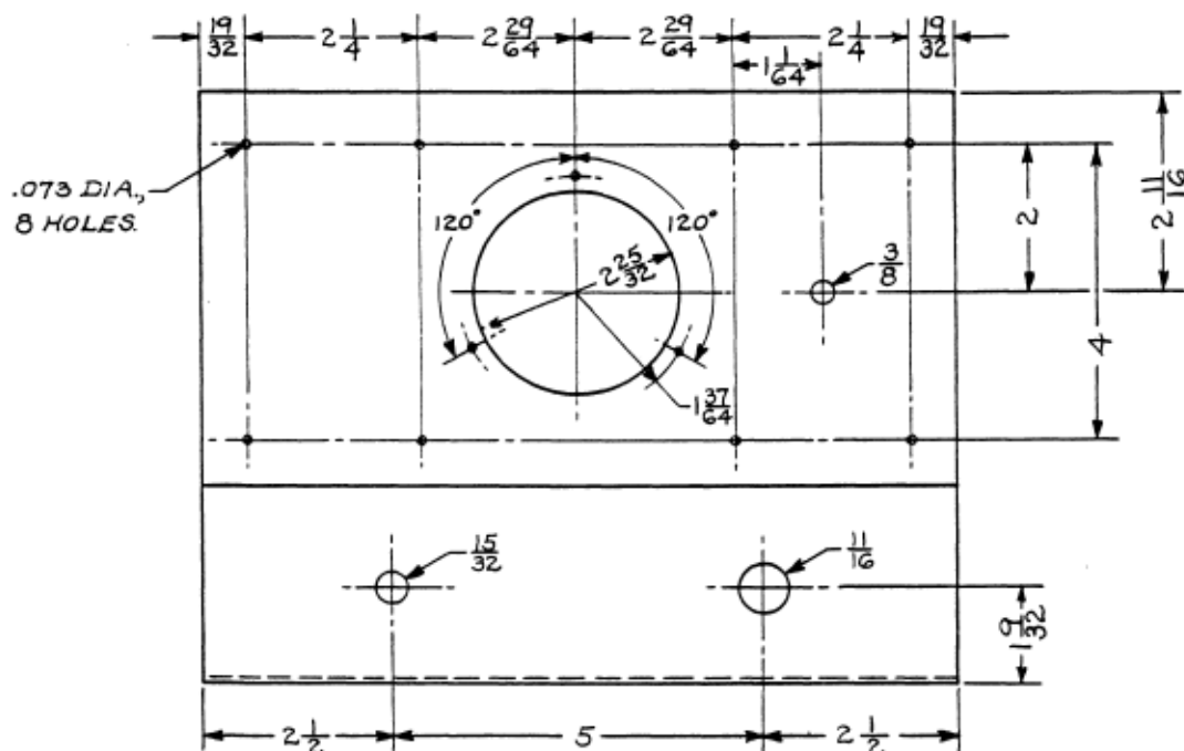
Figure 3C. HOUSING - MACHINED
