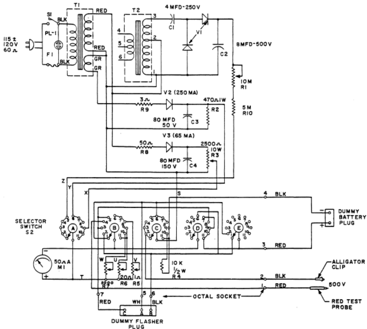
Figure 3A. SUPER GRAPHIC ANALYZER - SCHEMATIC DIAGRAM
