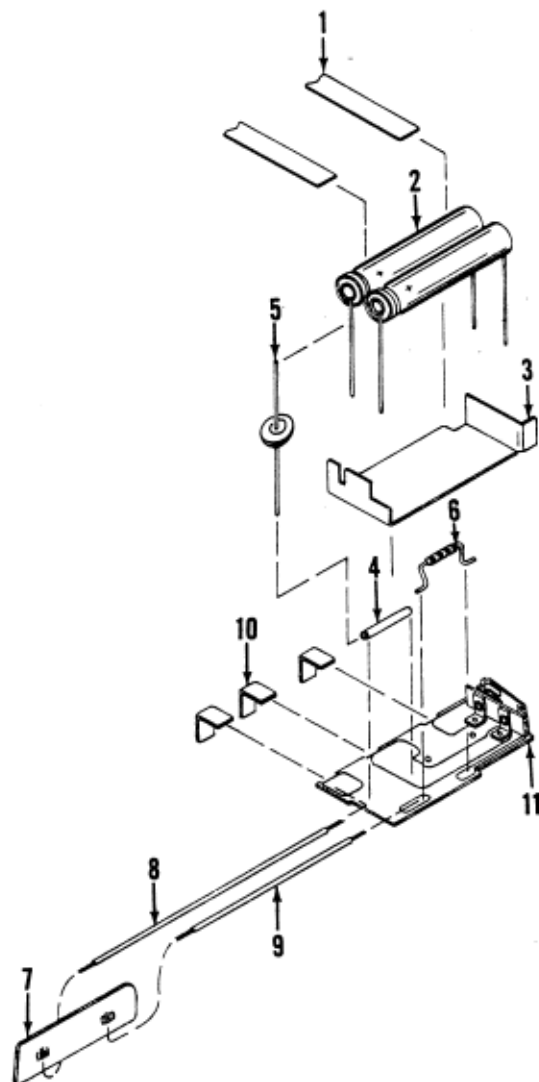
Figure 11A. CIRCUIT PLATE COMPLETE
