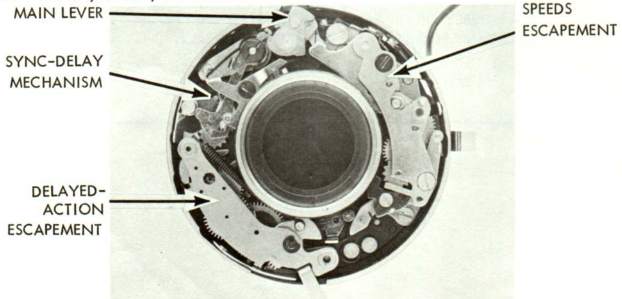
00-SIZE COPAL SV
