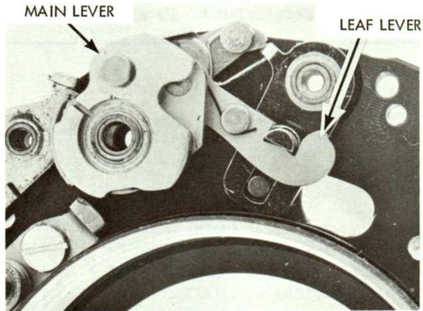
FIGURE 1 COPAL NO. 0
