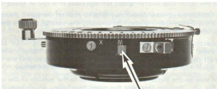
SYNC-CONTROL LEVER
