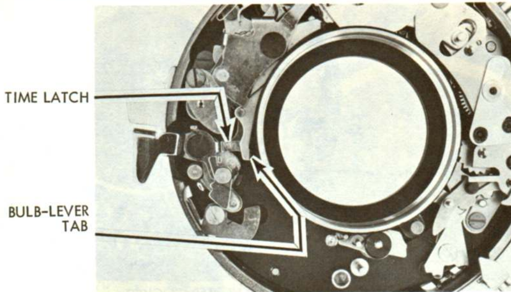
SHUTTER HELD OPEN ON "TIME"
