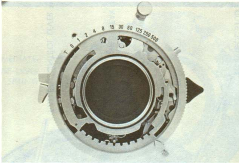
FIGURE 13 1/15 - SECOND SETTING
