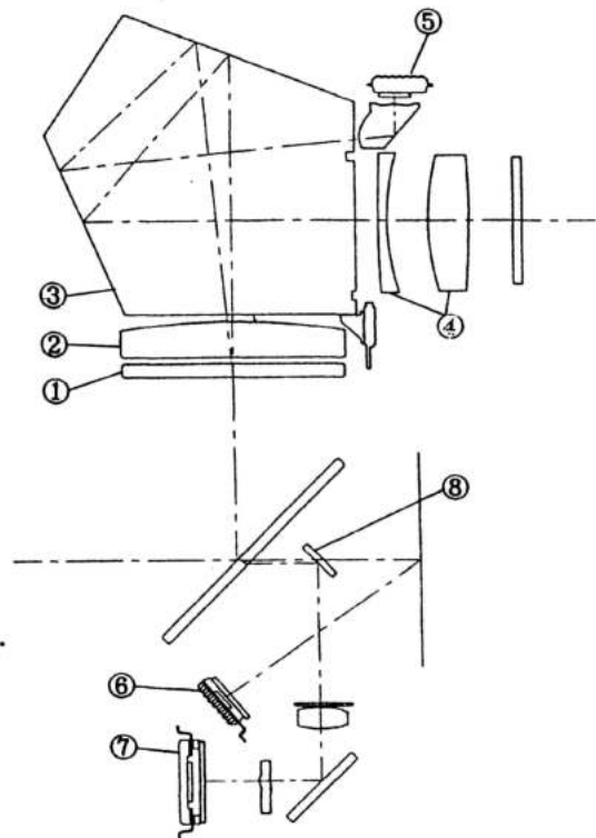
Fig.5 Optical System Layout
