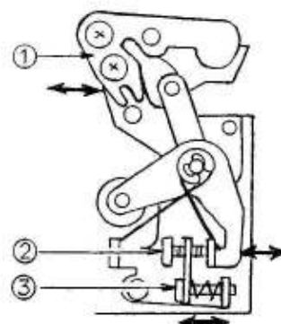
(ML Base Plate Ass'y)
