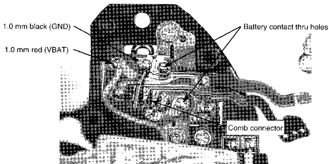
Figure 3-20 Battery Contact
