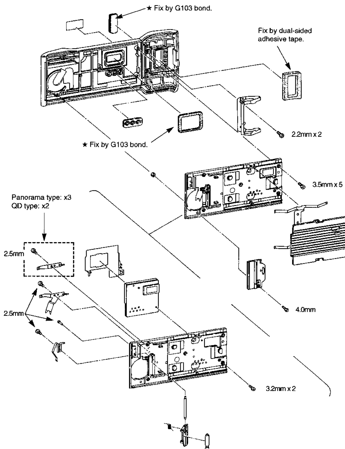
Figure 3-35 Back Cover Unit
