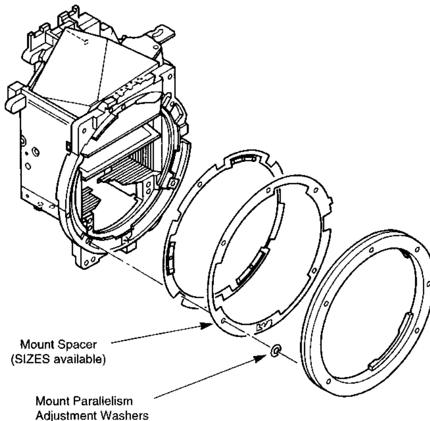
Figure 3-45 Flange Back Adjustment
