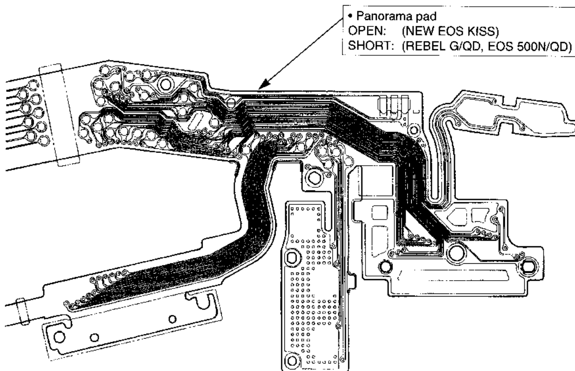
Figure 3-27 Panorama Pad
