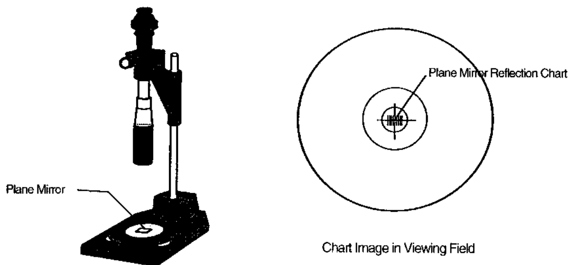
Figure 3-37 Auto Collimator
