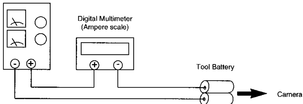
Fig. 3-3 Current Consumption Test Setup
