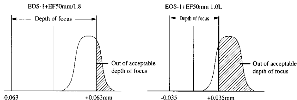
Fig. 3-58 Minute Defocus
