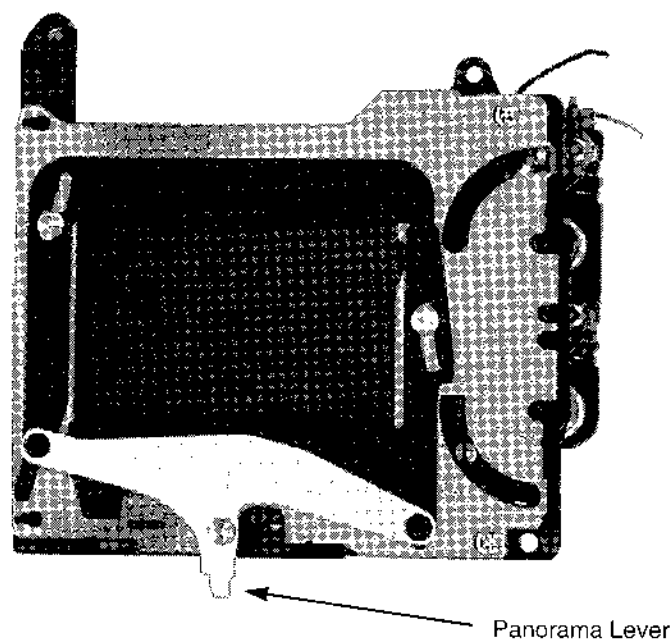
Figure 3-24 Shutter Unit
