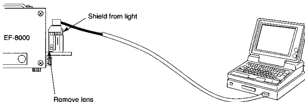
Fig. 3-55 AGC Adjustment
