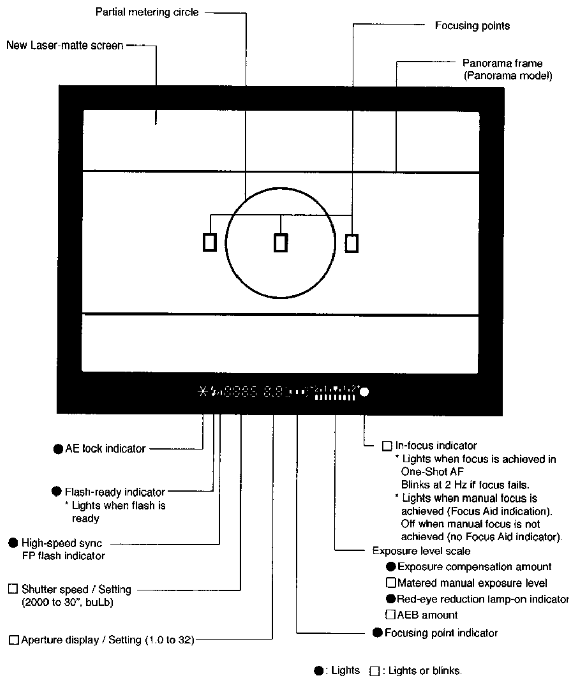
Fig. 1-2 Viewfinder Indicators
