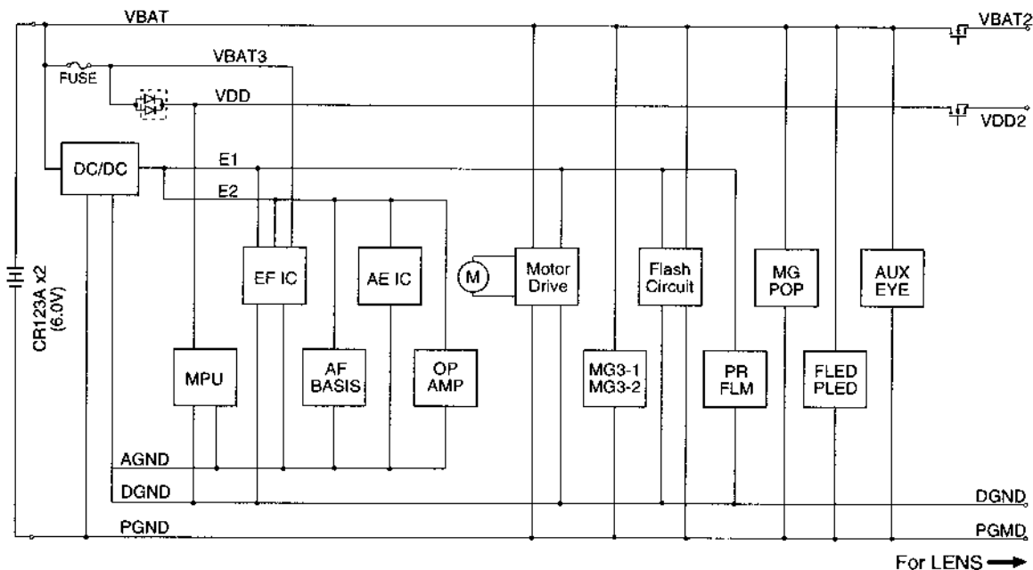
Fig. 2-9 Power Distribution
