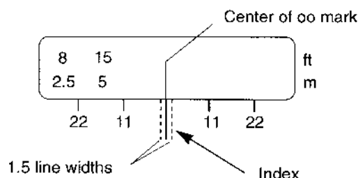
Figure 3-46 Lens Focusing Scale and Index
