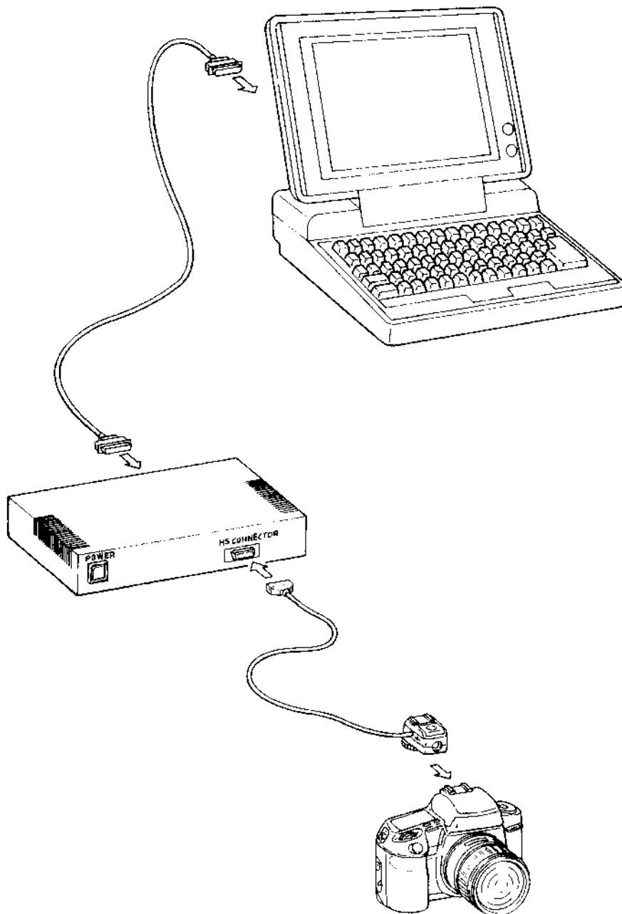
Fig. 3-48 Camera Connection
