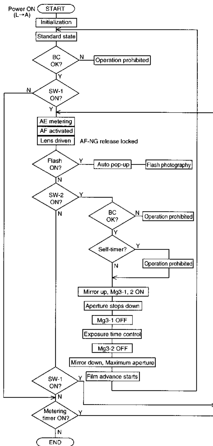
Fig. 2-7 Sequence Flow (normal photography)
