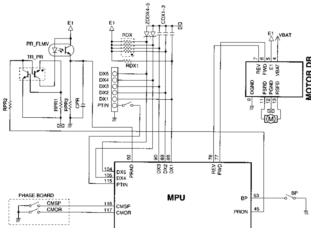
Fig. 2-11 Film Transport
