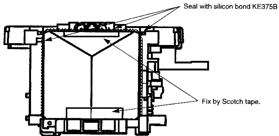
Figure 3-31 Pentamirror Installation
