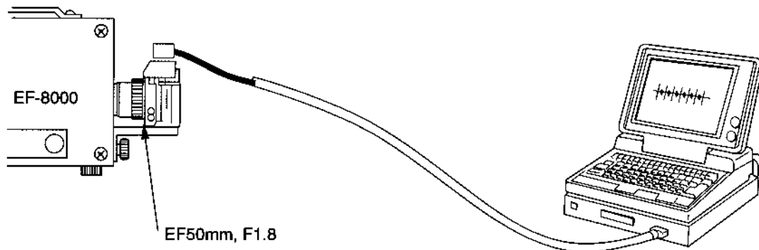
Fig. 3-50 Shutter Adjustment
