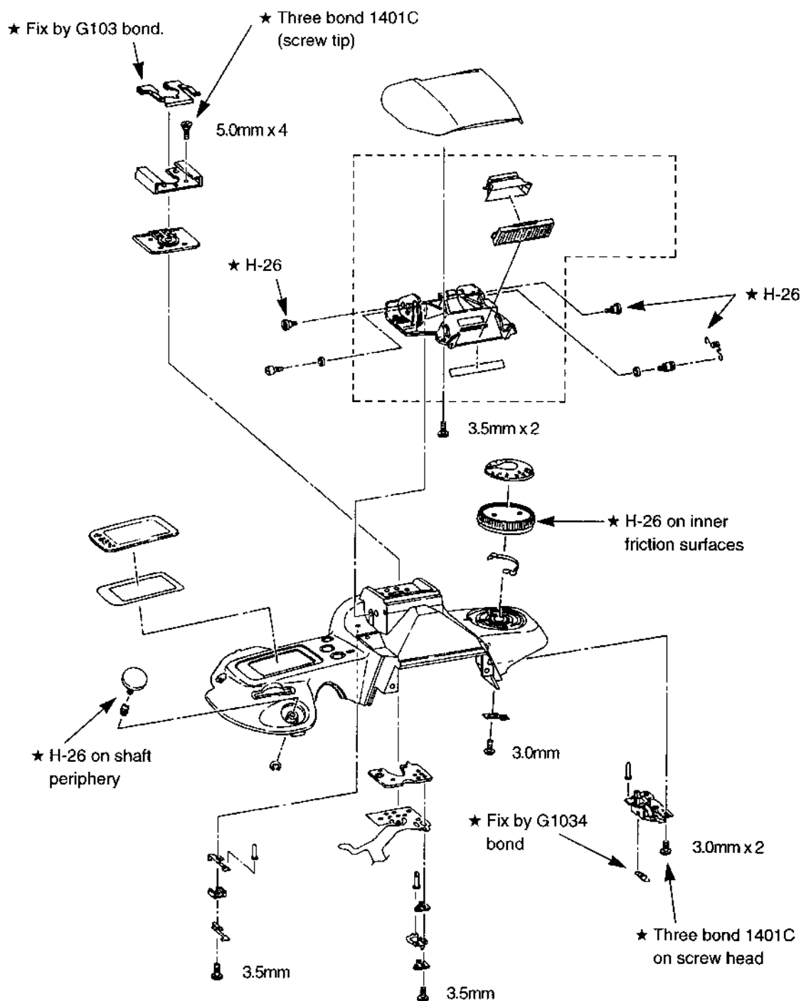
Figure 3-36 Top Cover Unit
