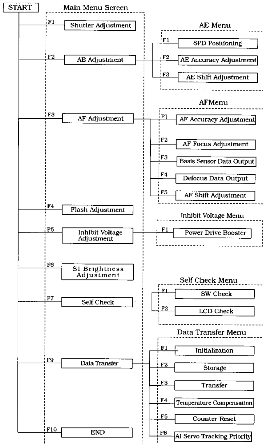
Fig. 3-86 Adjustment Items
