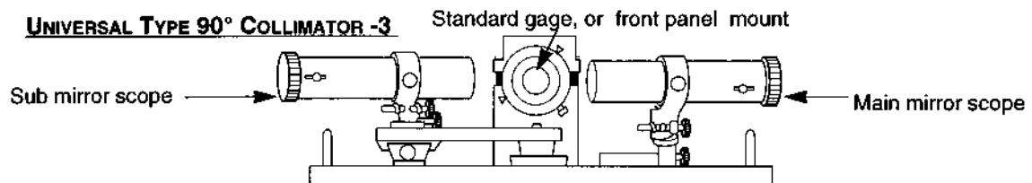
Fig. 3-54 90° Collimator Adjustment
