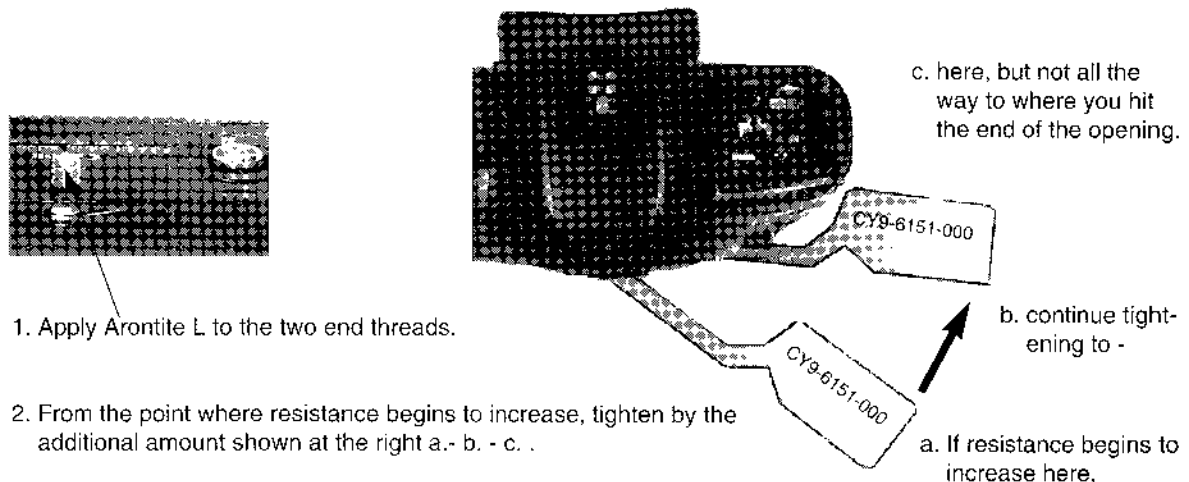
Fig. 3-01a Nut Tightening Procedure
