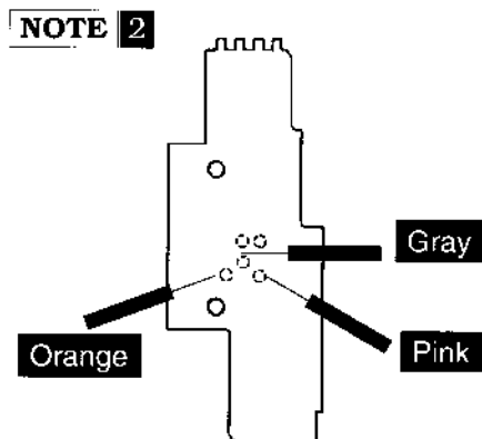
Fig. 3-19 DC/DC Leads
