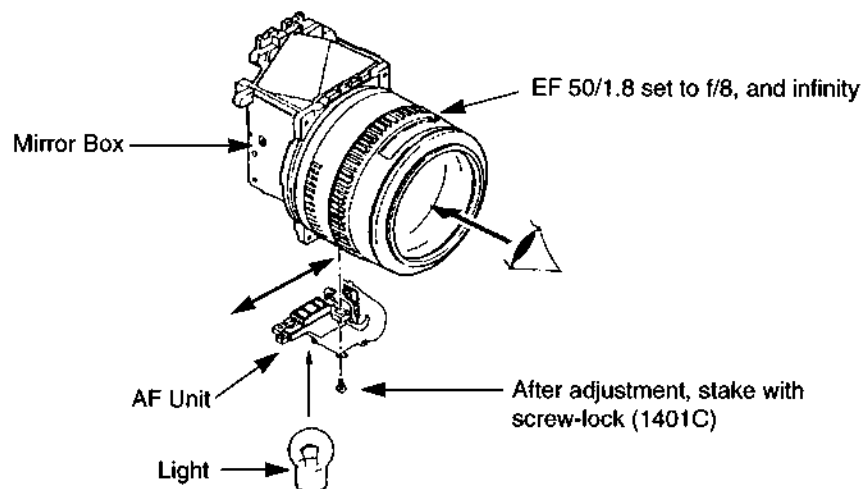
Fig. 3-58 BASIS Positioning
