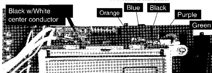
Fig. 3-15 Electronic Dial Lead Removal
