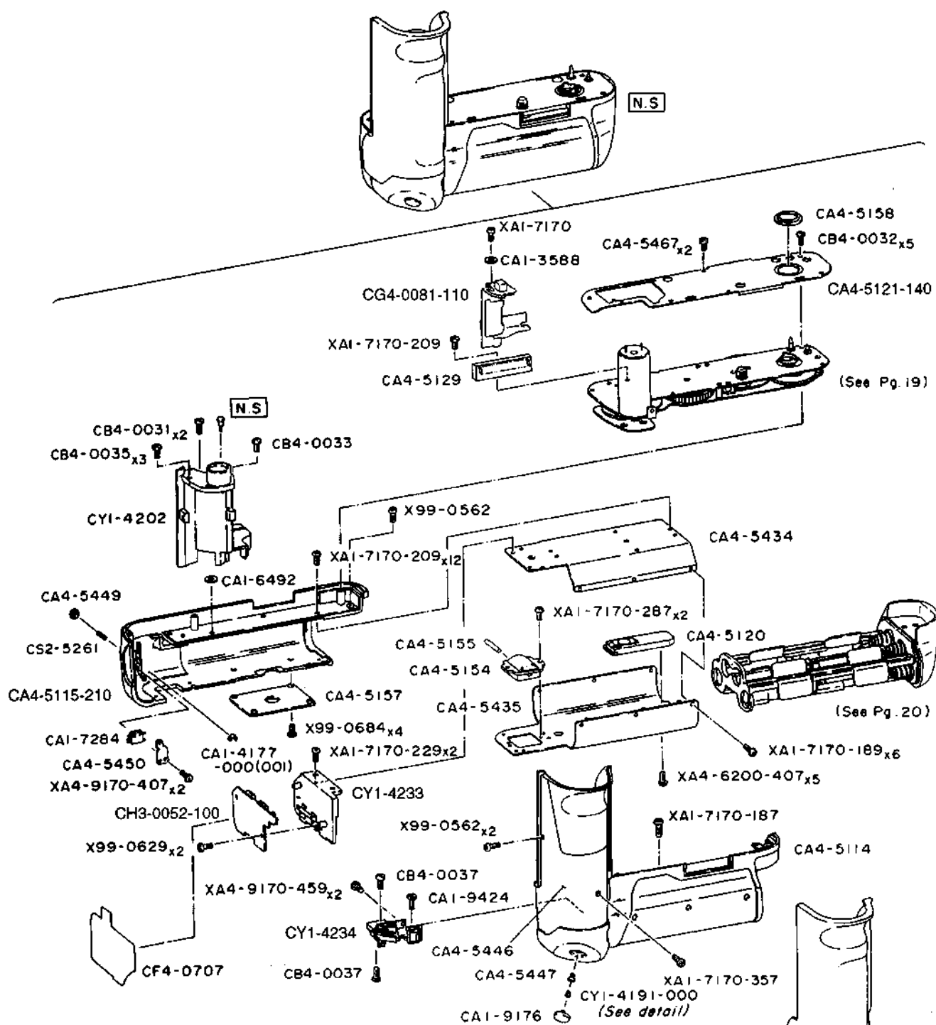
CY1-4191-000 detail (STANDARD)
