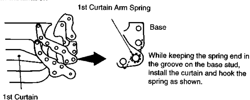
Fig. 3-49 1st Curtain
