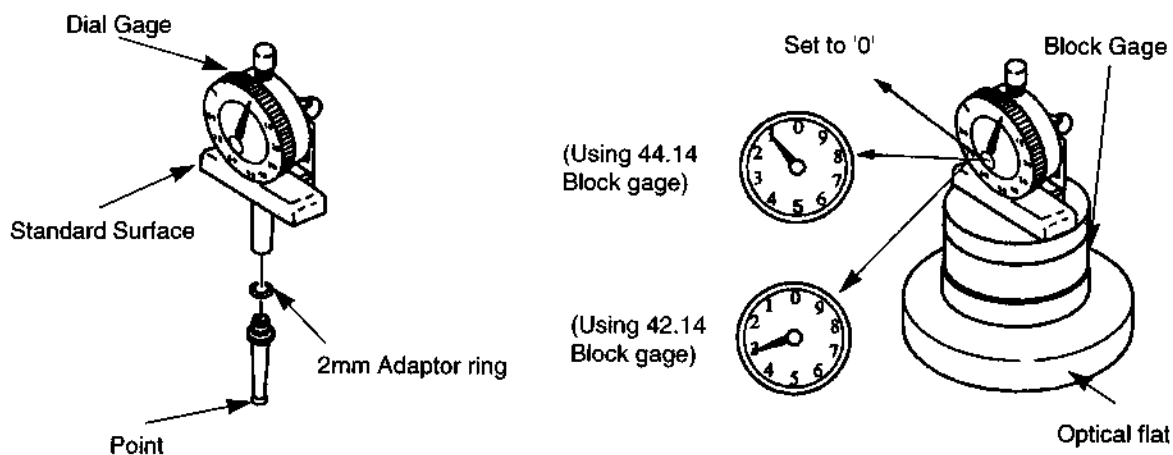
Fig. 3-65 Dial Gages
