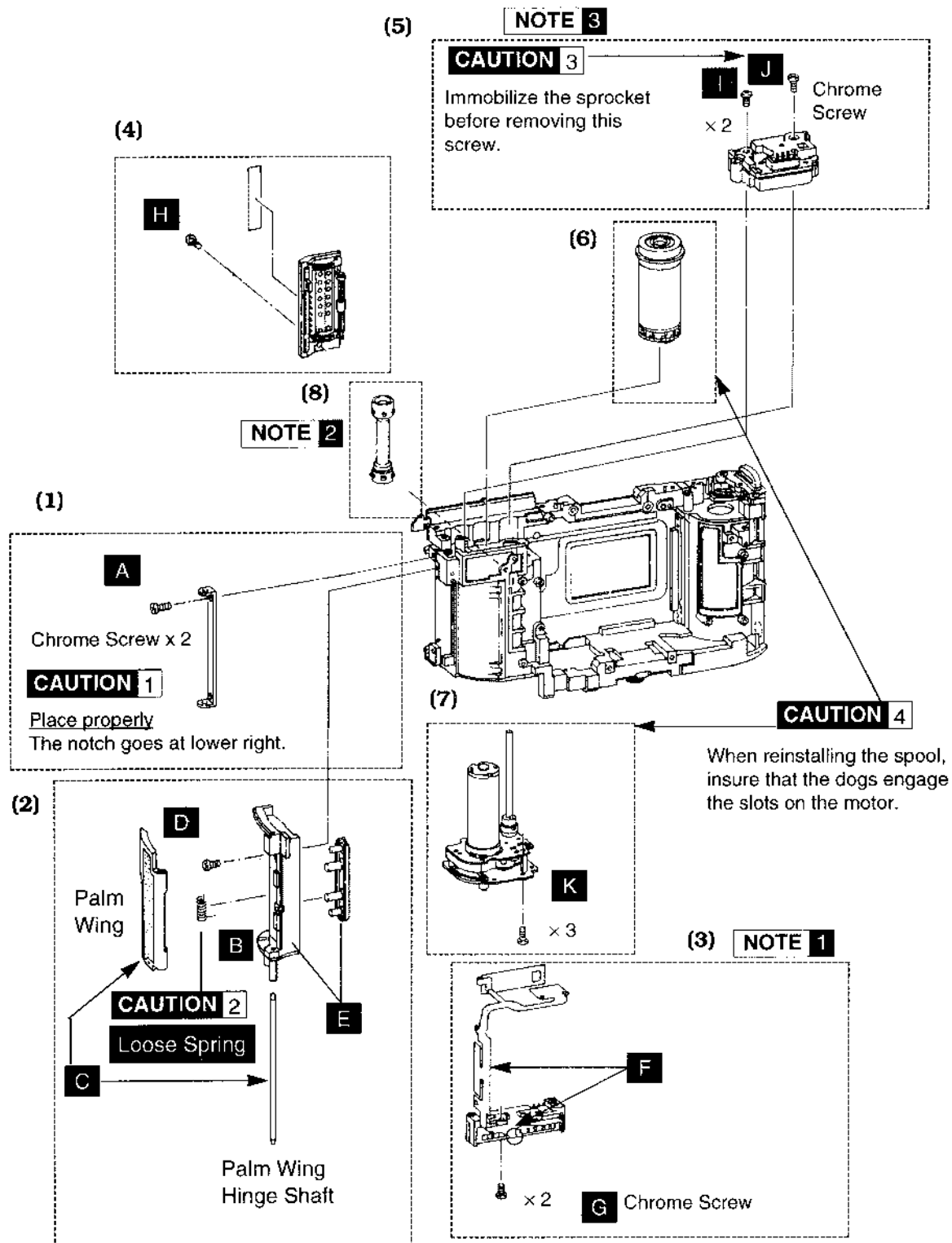
Fig. 3-22 Film Transport Parts Removal
