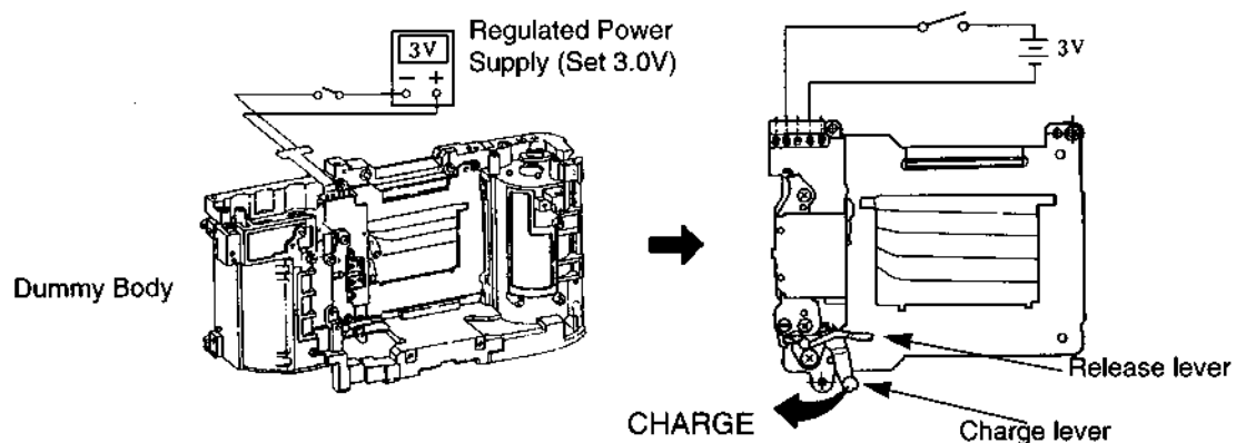
Fig. 3-61 Shutter Preparation
