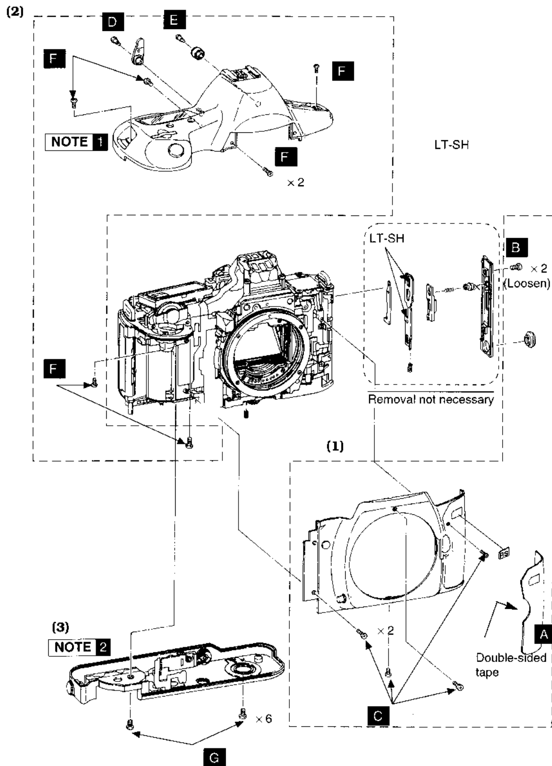
Fig. 3-02 External Covers Removal
