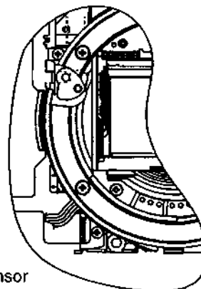
Fig. 3-41 Lead Dress
