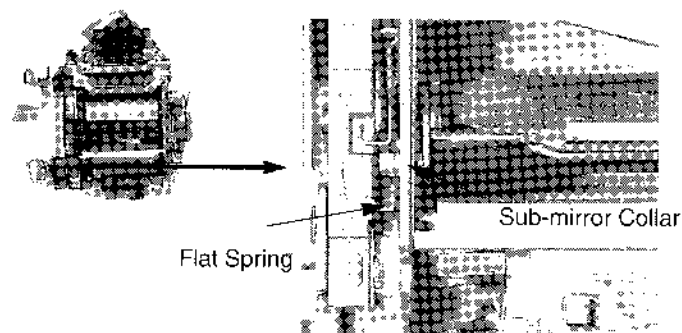
Fig. 3-30 Sub-mirror Installation
