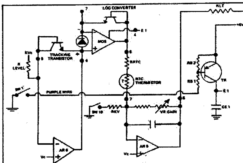
Light-measuring circuit
