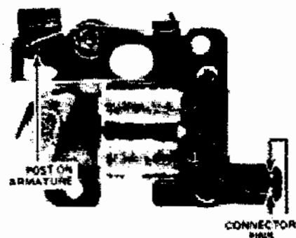
Figure 22 Combination-magnet assembly
