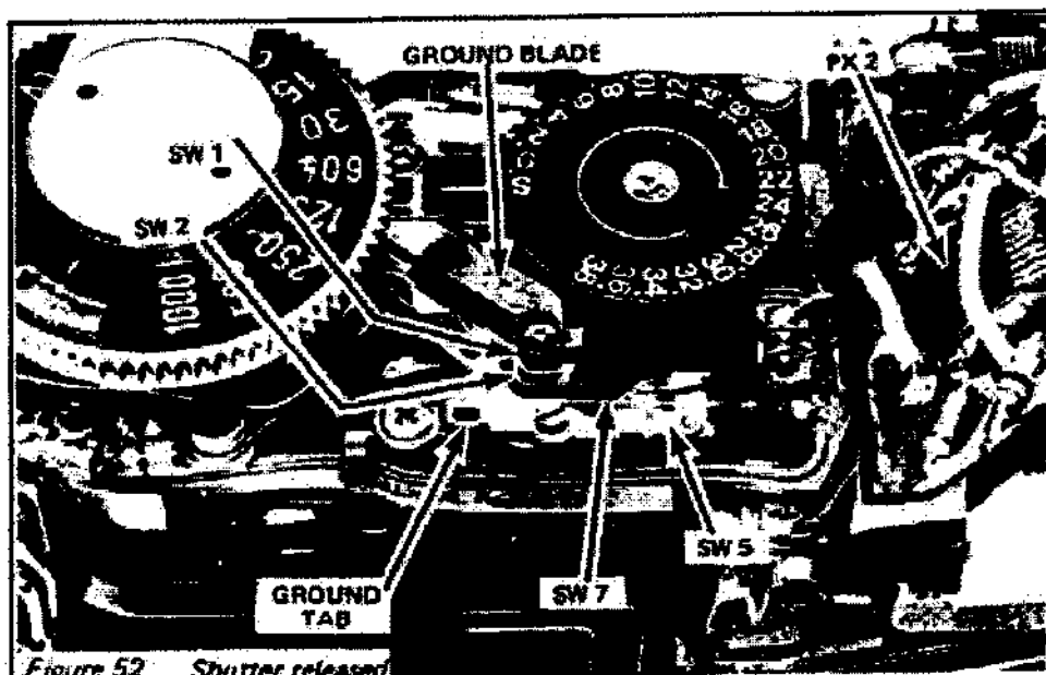
Figure 52 Shutter released
