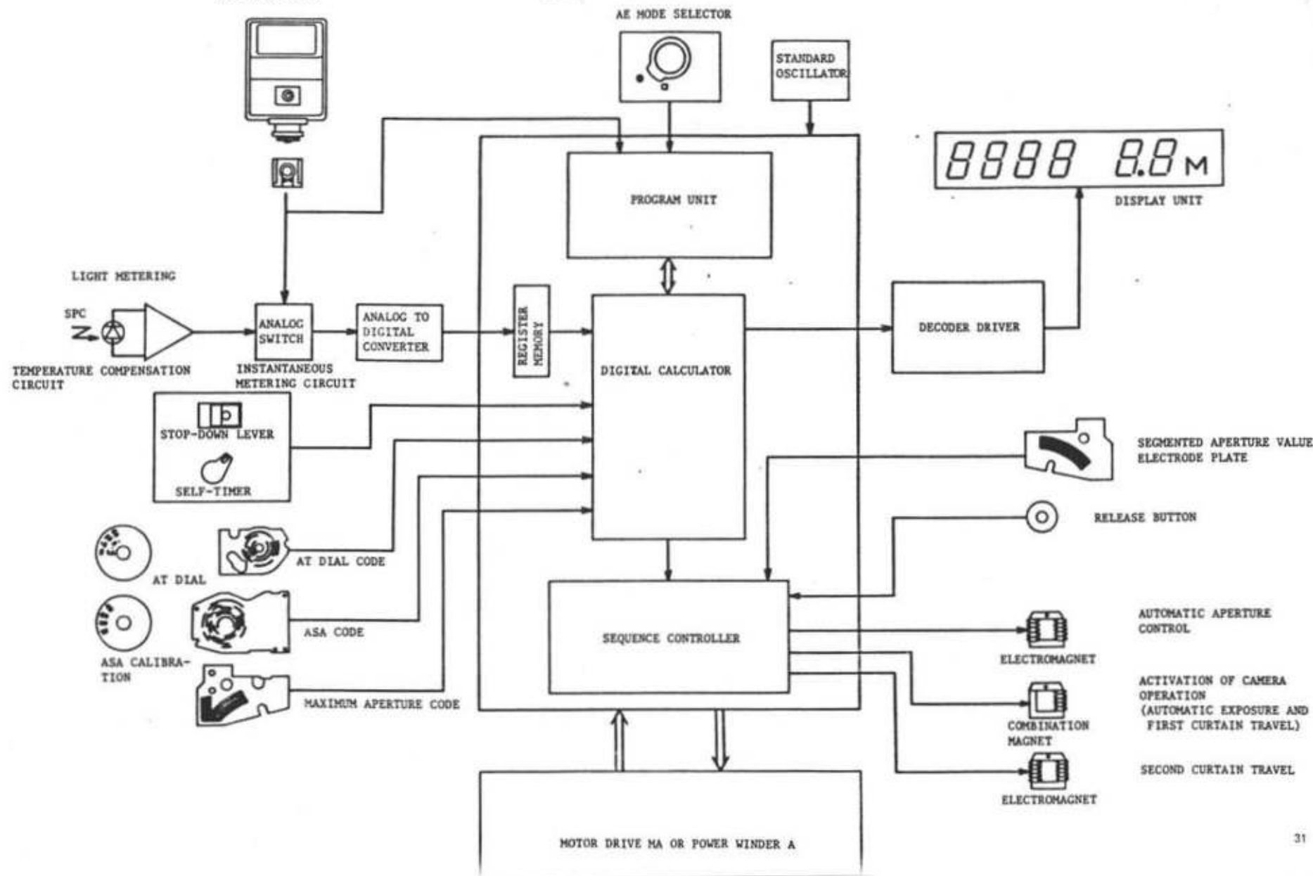
Fig. 6 2 BLOCK DIAGRAM OF COMPUTER INTEGRATED INTO CONTROL SYSTEM
