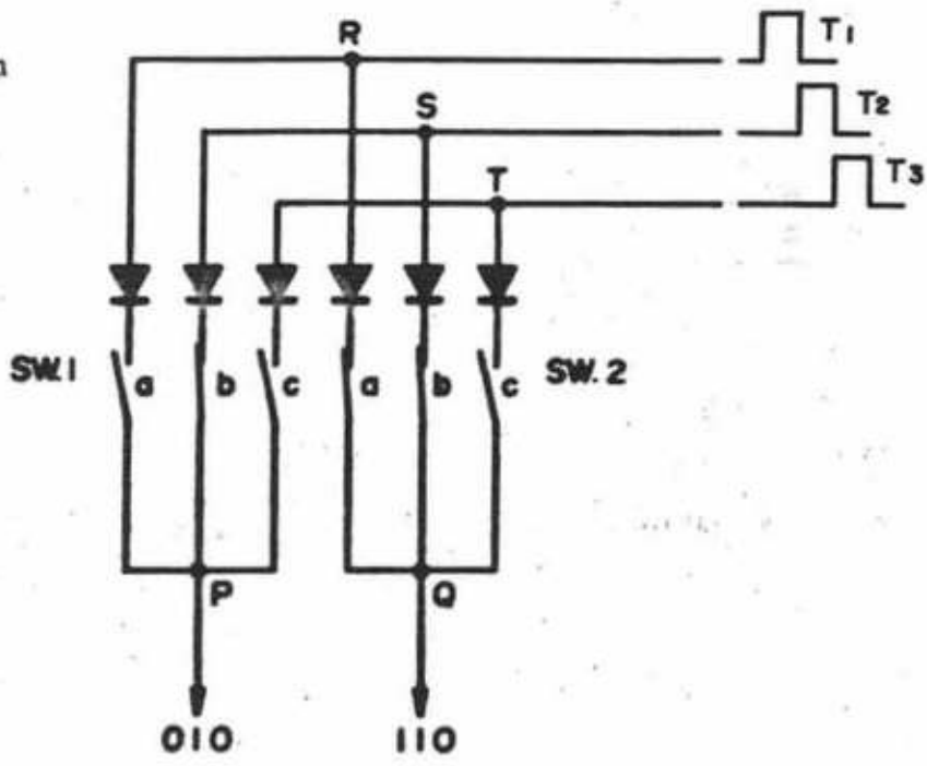
Fig. 20 Diode Array Diagram
